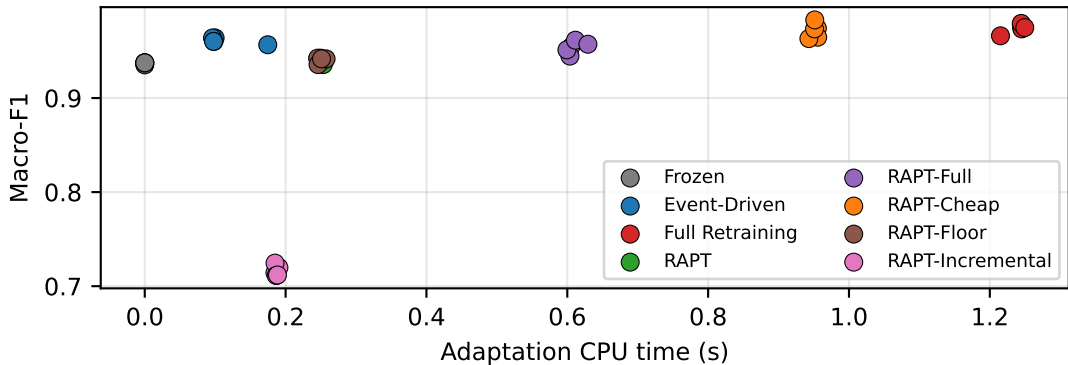
5G Campus — accuracy vs adaptation cost (per seed)
